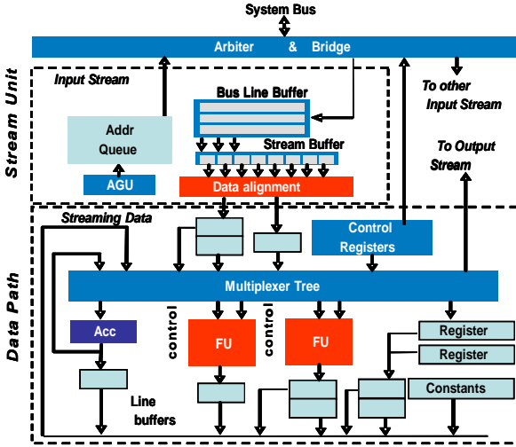
Figure 2. Streaming accelerator template with Stream Unit and Data Path
