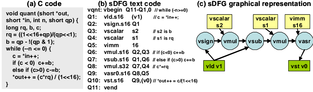
Figure 1. Example program in (a) C notation, (b) sDFG text, and (c) graphical notation
